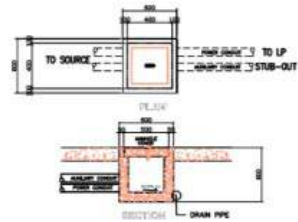
HANDHOLE DETAIL
