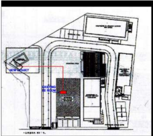
SITE DEVELOPMENT PLAN
