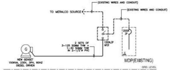
POWER SINGLE LINE DIAGRAM
